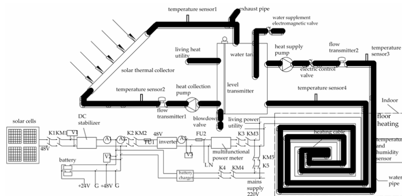
Figure 15. The overall design of the system [29]
