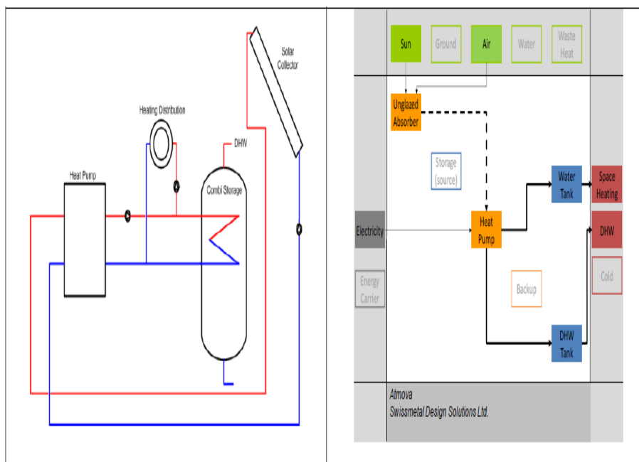
Figure 14. Unified (left) hydraulic and square (right) SHPS view. An unglazed collector is only used as the heat source for the heat pump in this system.
