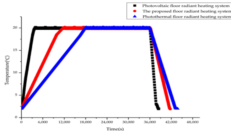
Figure (16): "Indoor temperature changes of the three different heating systems[29]."
