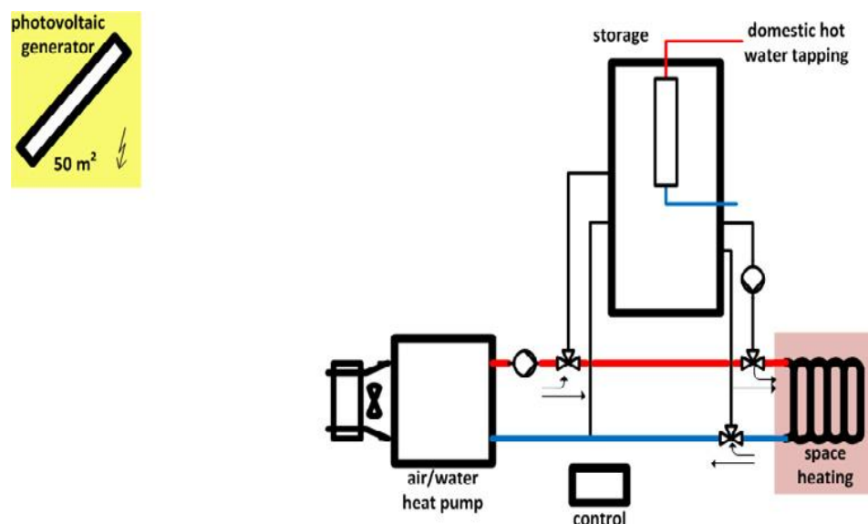
Figure 8. Heat pump and photovoltaic system.
