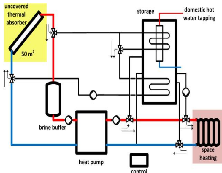
Figure 10. Uncovered thermal absorber with heat pump system.
