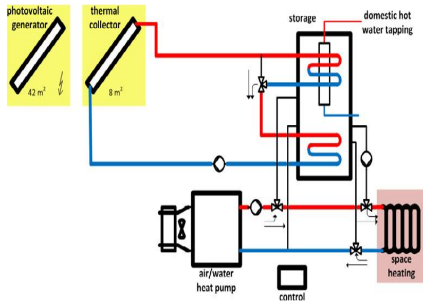
Figure 9. Small solar thermal side-by-side with a photovoltaic system.
