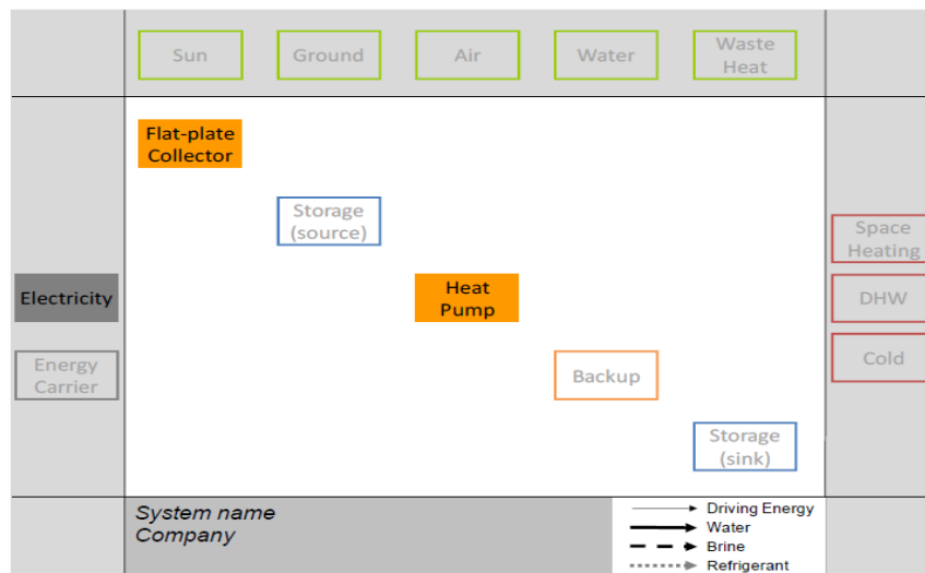
Figure 11. Diagram structure showing the main elements, heat sources, thermal sinks and another electricity carrier in a solar heat pump assisted system.
