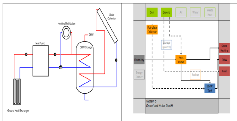
Figure 12. Unified (left) hydraulic system and an SHPS "square view" (right) visualization scheme. Geothermal heat is used as a heat source, whereas solar and heat pumps are only connected "parallel."
