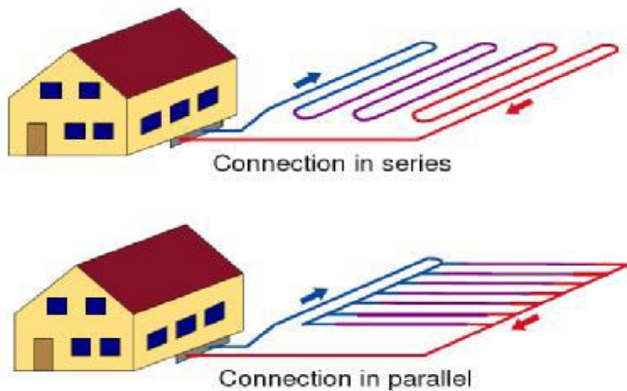
Figure (5): System of horizontal closed-loop
