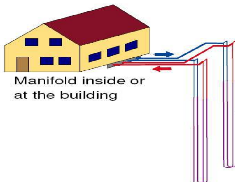
Figure 6. System of vertical closed-loop
