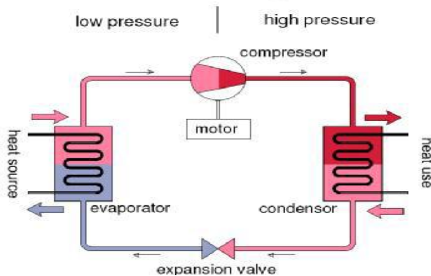
Figure 1. Diagram of a compression heat pump.
