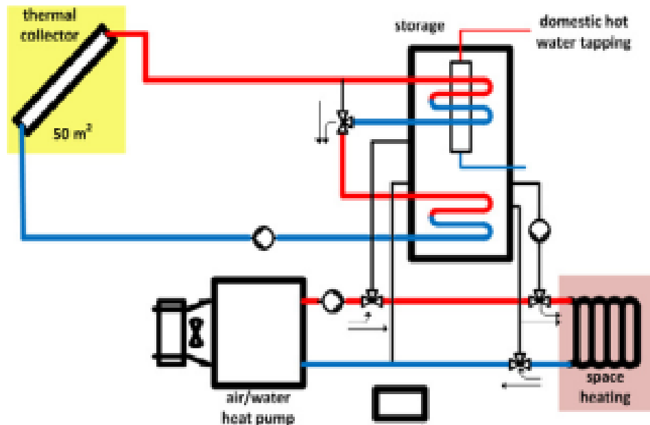
Figure 7. Direct solar heat generation.
