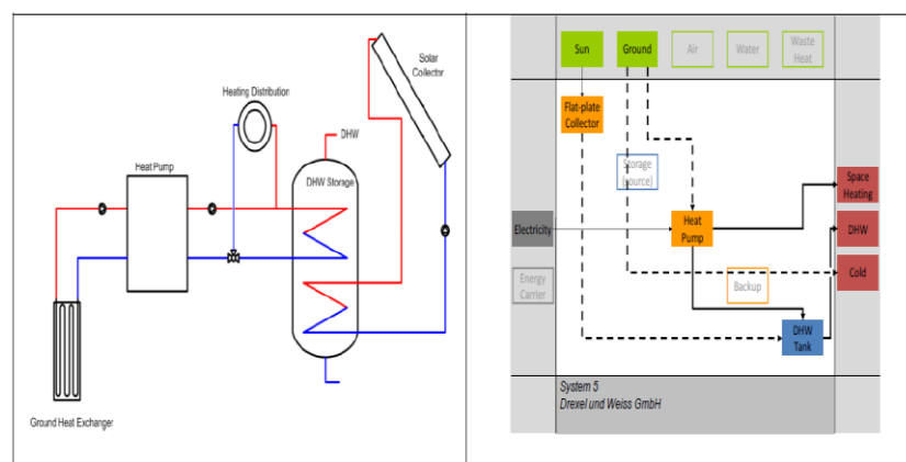
Figure 12. Unified (left) hydraulic system and an SHPS "square view" (right) visualization scheme. Geothermal heat is used as a heat source, whereas solar and heat pumps are only connected "parallel."
